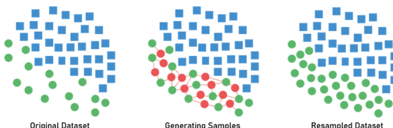
Figure 2.5: SMOTE
