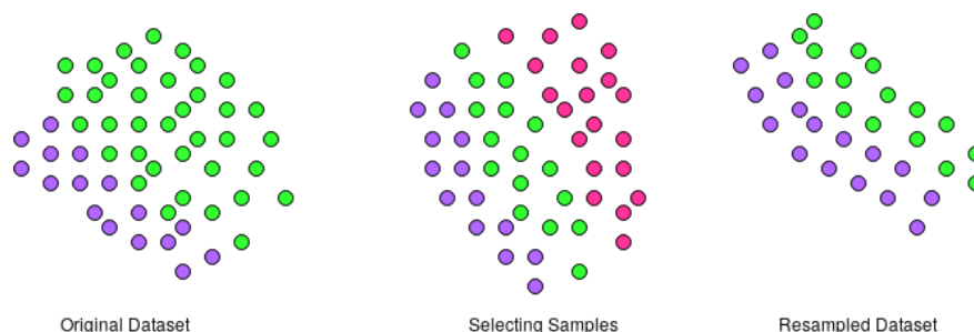
Figure 2.2: Nearmiss-3 Approach
