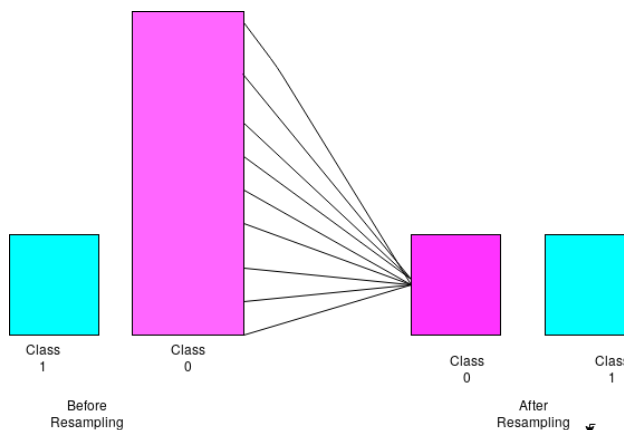
Figure 2.1: Undersampling approach
