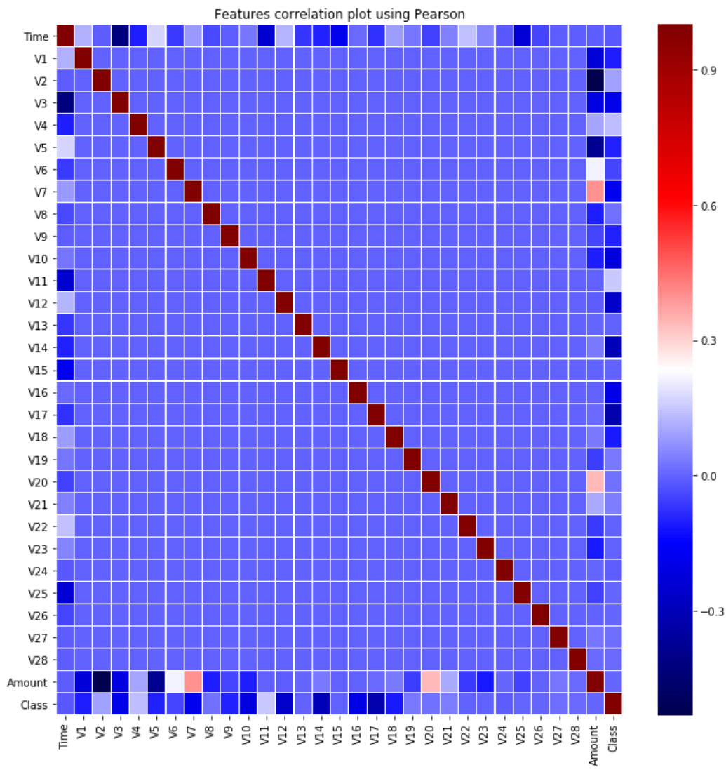
Figure 3.2: Correlation Matrix
