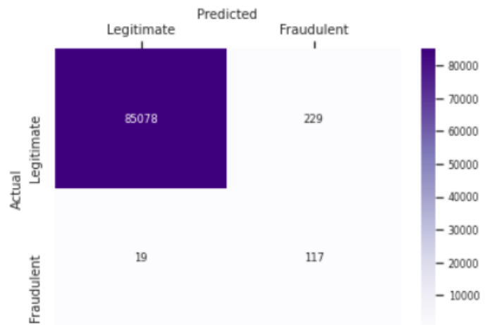
Figure 4.1: Confusion matrix-RF and Nearmiss
