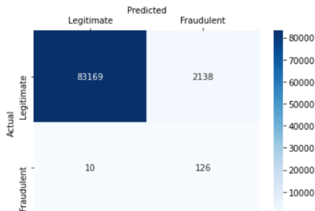
Figure 4.10: ConfMat-SVM and SMOTE+Tomek
