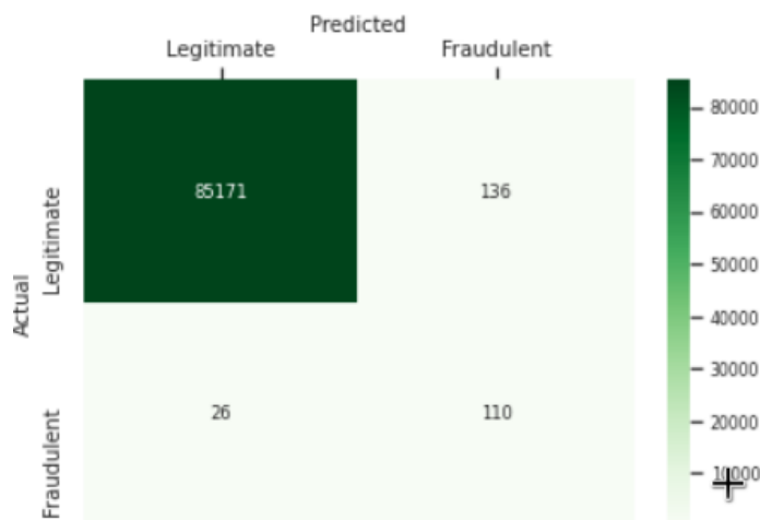
Figure 4.4: Confusion Matrix-KNN and Nearmiss
