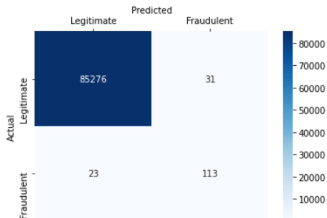
Figure 4.12: Confusion Matrix-SVM and ENN+CNN
