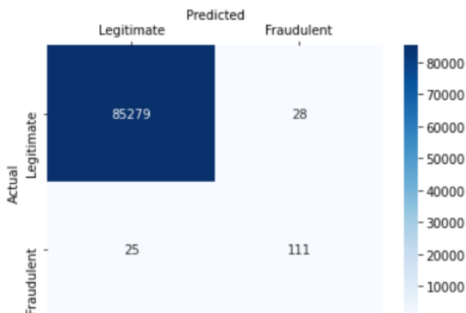
Figure 4.11: Confusion Matrix-SVM and Nearmiss
