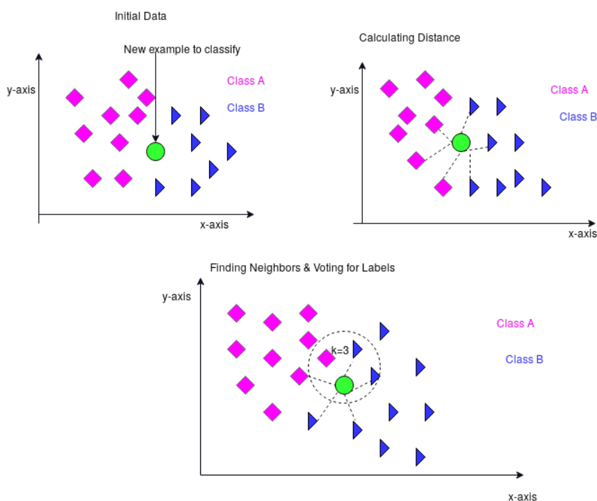
Figure 2.7: How KNN classifies the new instance
